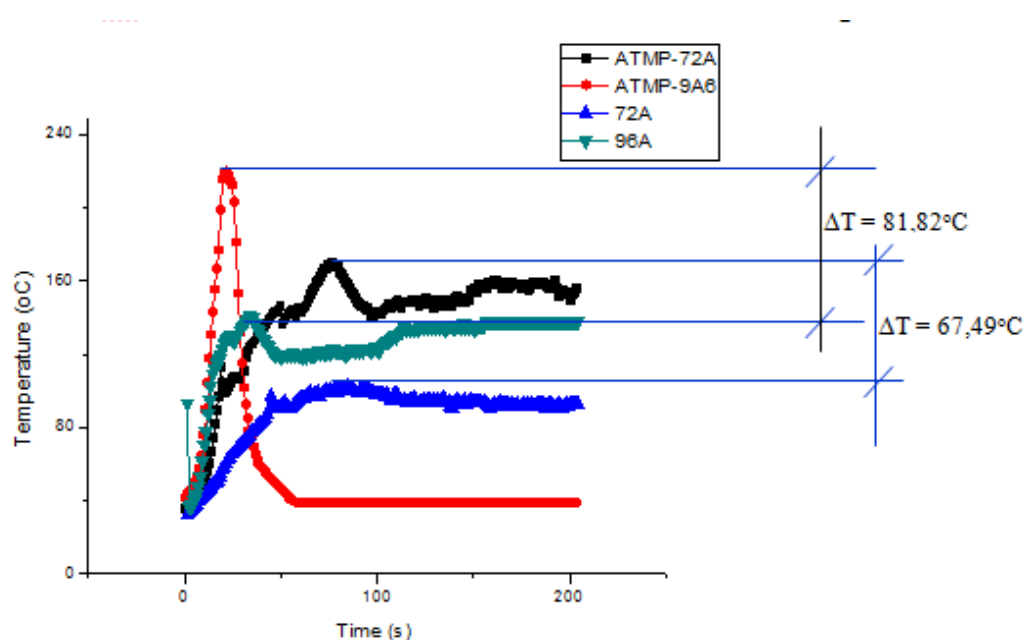
Figure 8 Comparison when cable loaded with 72 A and 96 A at atmospheric vs. oxygen concentration 15%
