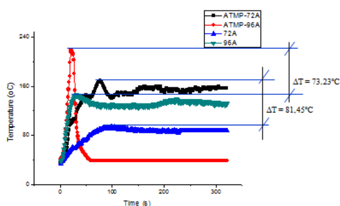
Figure 5 Comparison when cable loaded with 72 A and 96 A at atmospheric vs. oxygen concentration 19%
