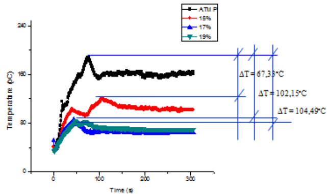
Figure 10 Comparing cable temperature at 72 A at atmospheric and oxygen concentration 15%–19%
